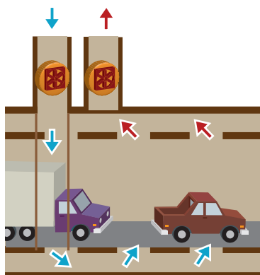
Transverse Ventilation
