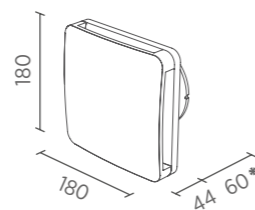
ALBA 12/5" Ø 120 mm
